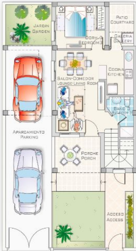
Planta Baja / Ground Floor
